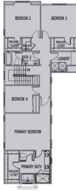
SECOND FLOOR
