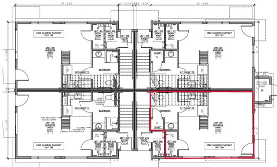
2352 VAQUERO PARKWAY - MAIN LEVEL PLAN
