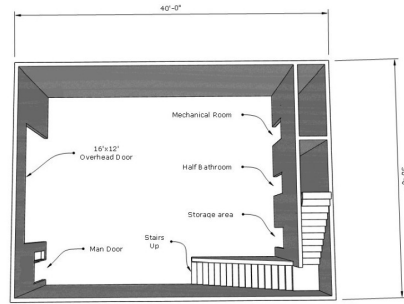
Arden Drive Plan 1 Main Floor 1200 sq. ft. Shop/Garage
