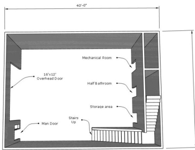
Arden Drive Plan 1 Plan Floor 1200 sq. ft. Shop/Garage
